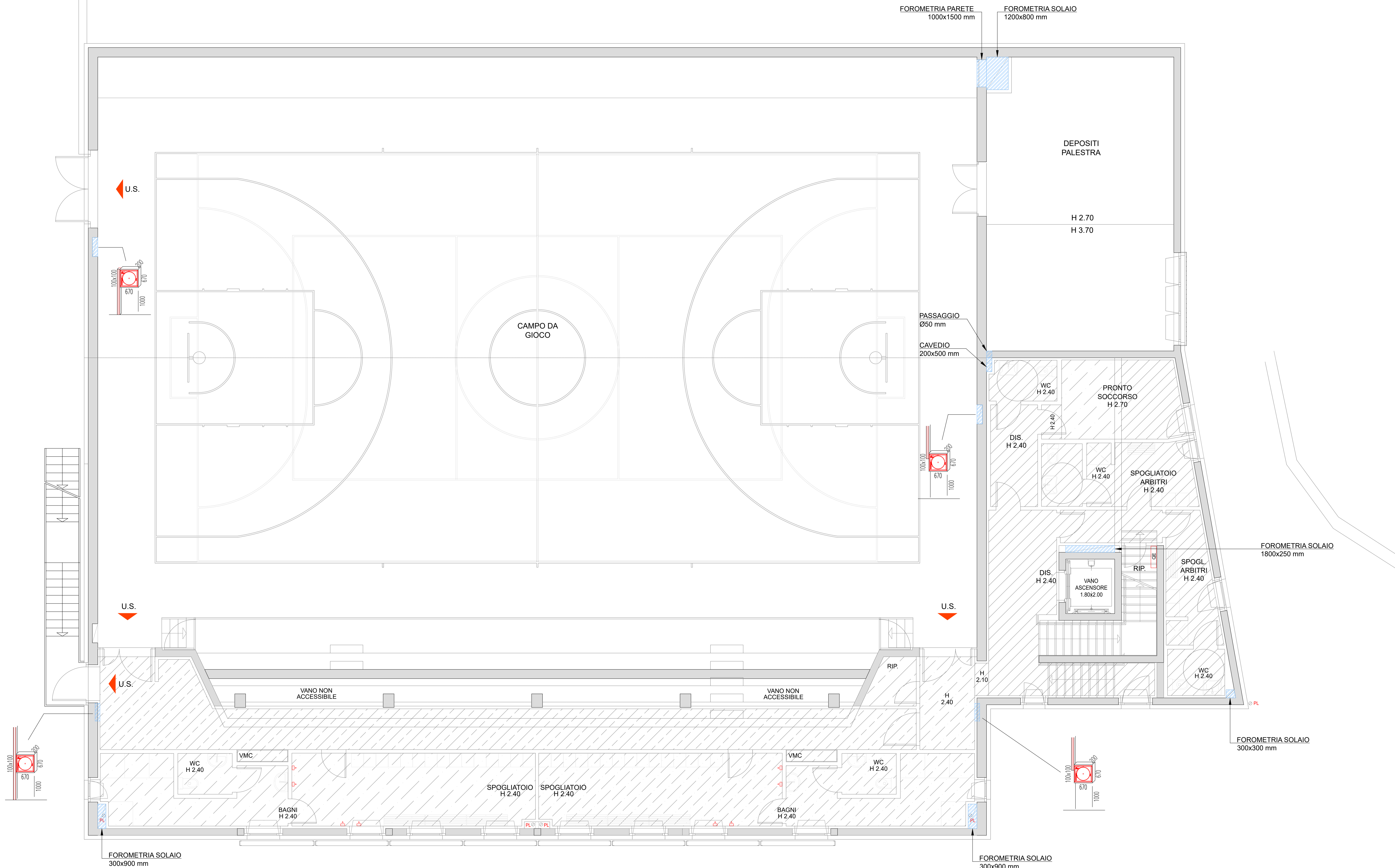
PIANTA PIANO +6,10
